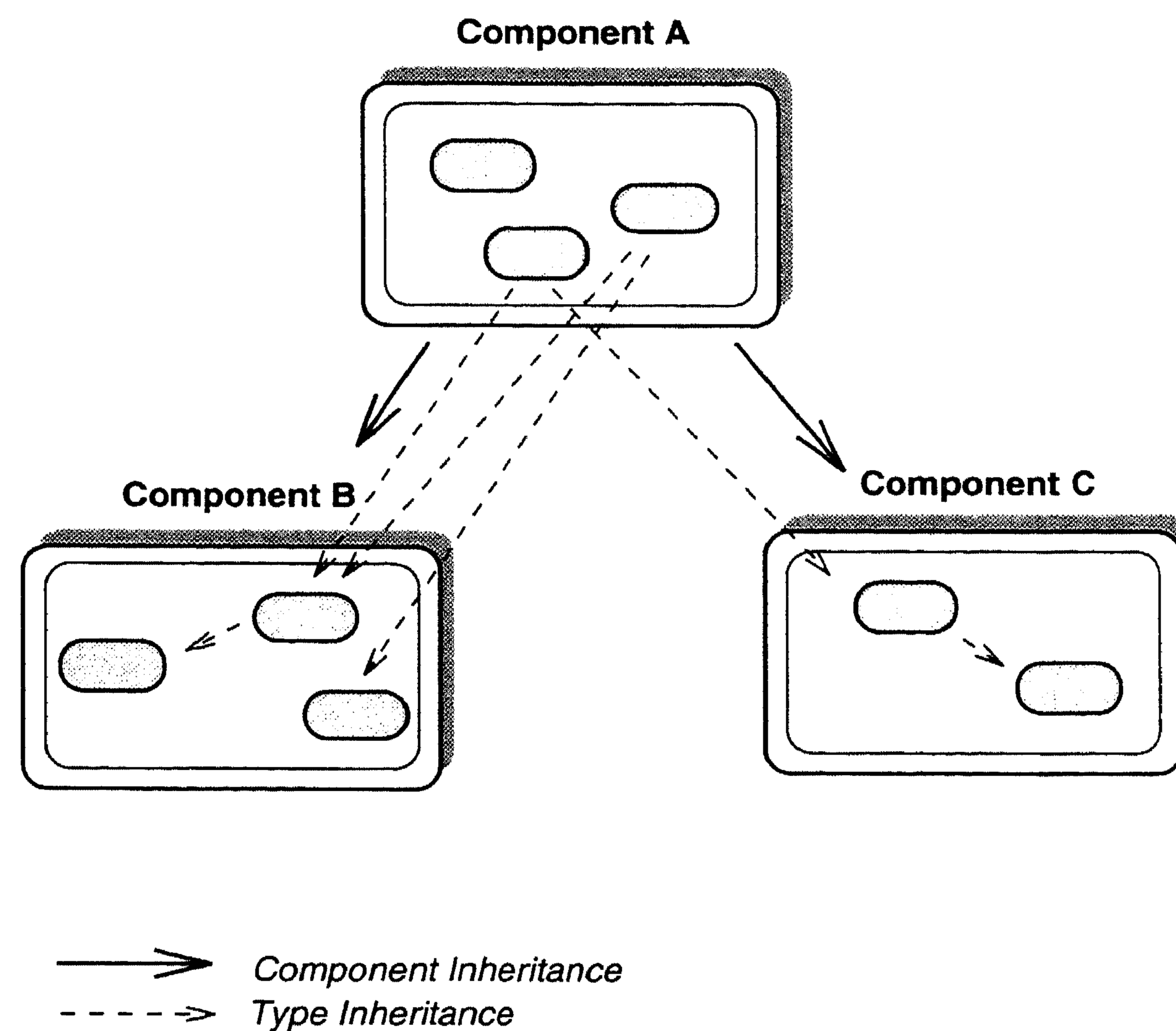
FIGURE 1. Component inheritance.
